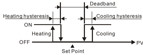
Figure 4: ON/OFF Control
